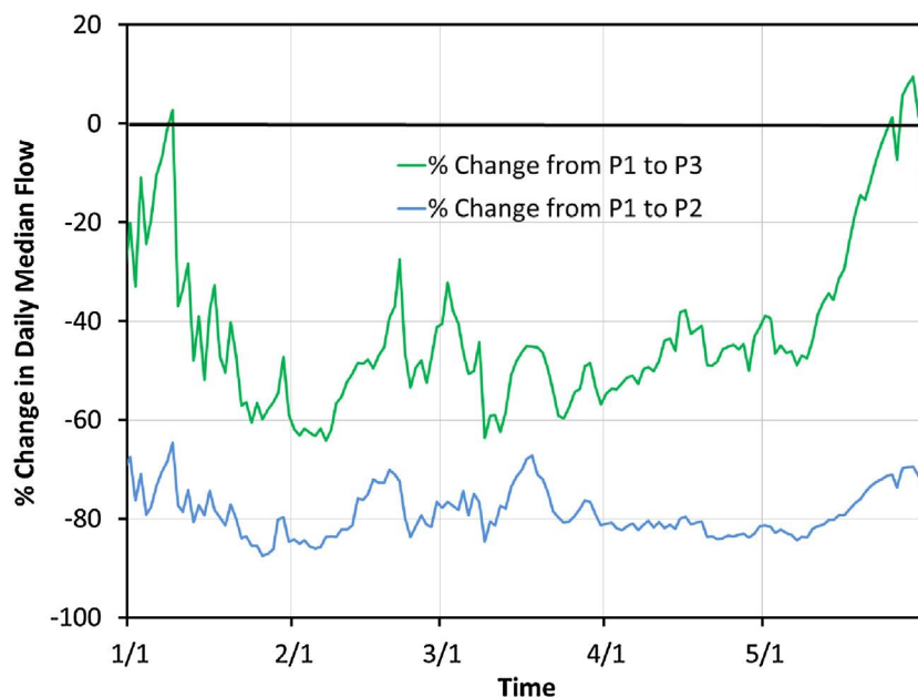
Fig. 5. Percent change in median daily flows in Clear Creek from the pre-project period (P1: 1941–1958) to the first post-project period (P2: 1965–1994) or the second post-project period (P3: 1995–2013).
