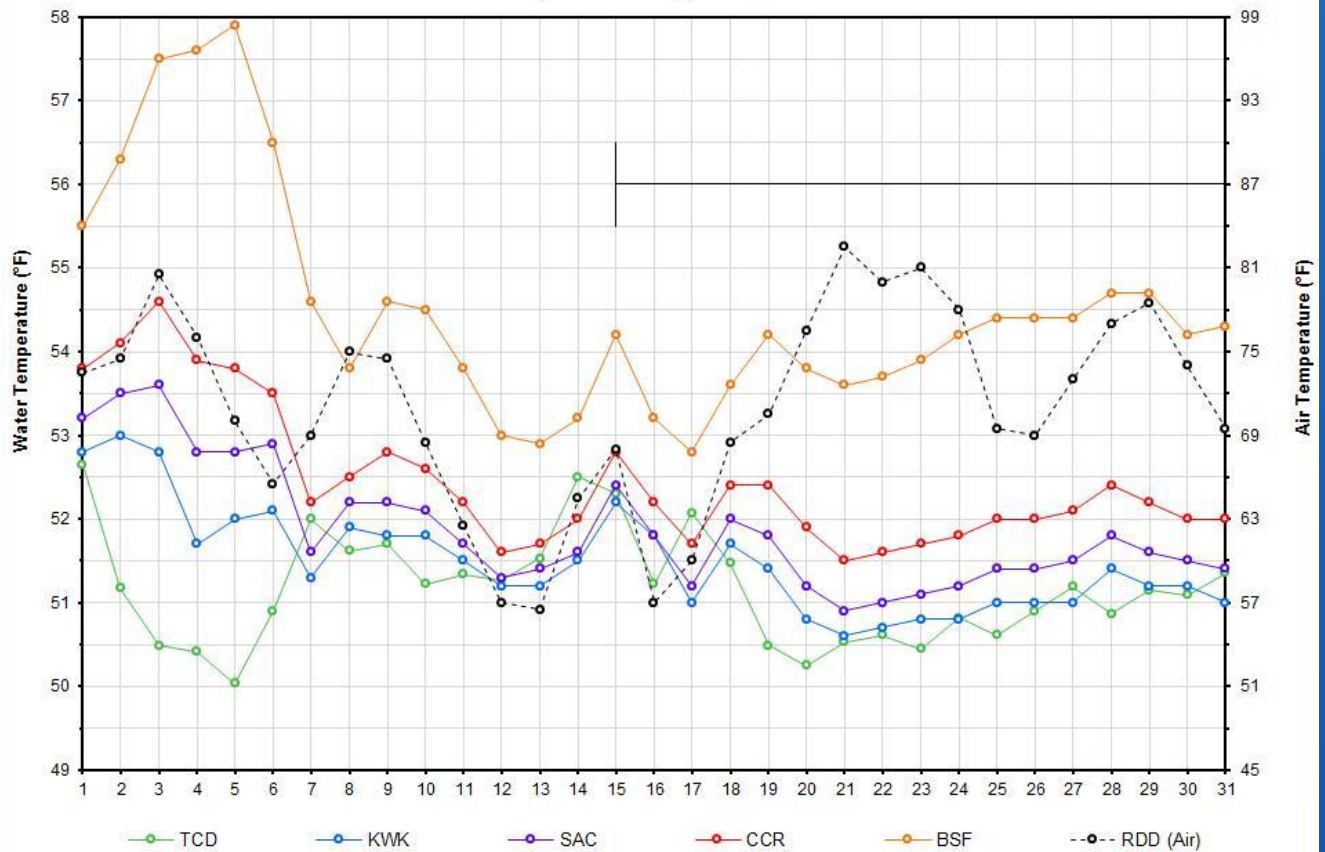
May Mean Daily Temperatures
