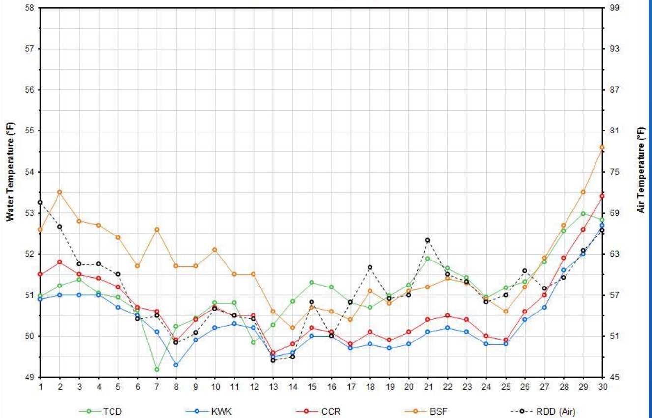
April Mean Daily Temperatures
