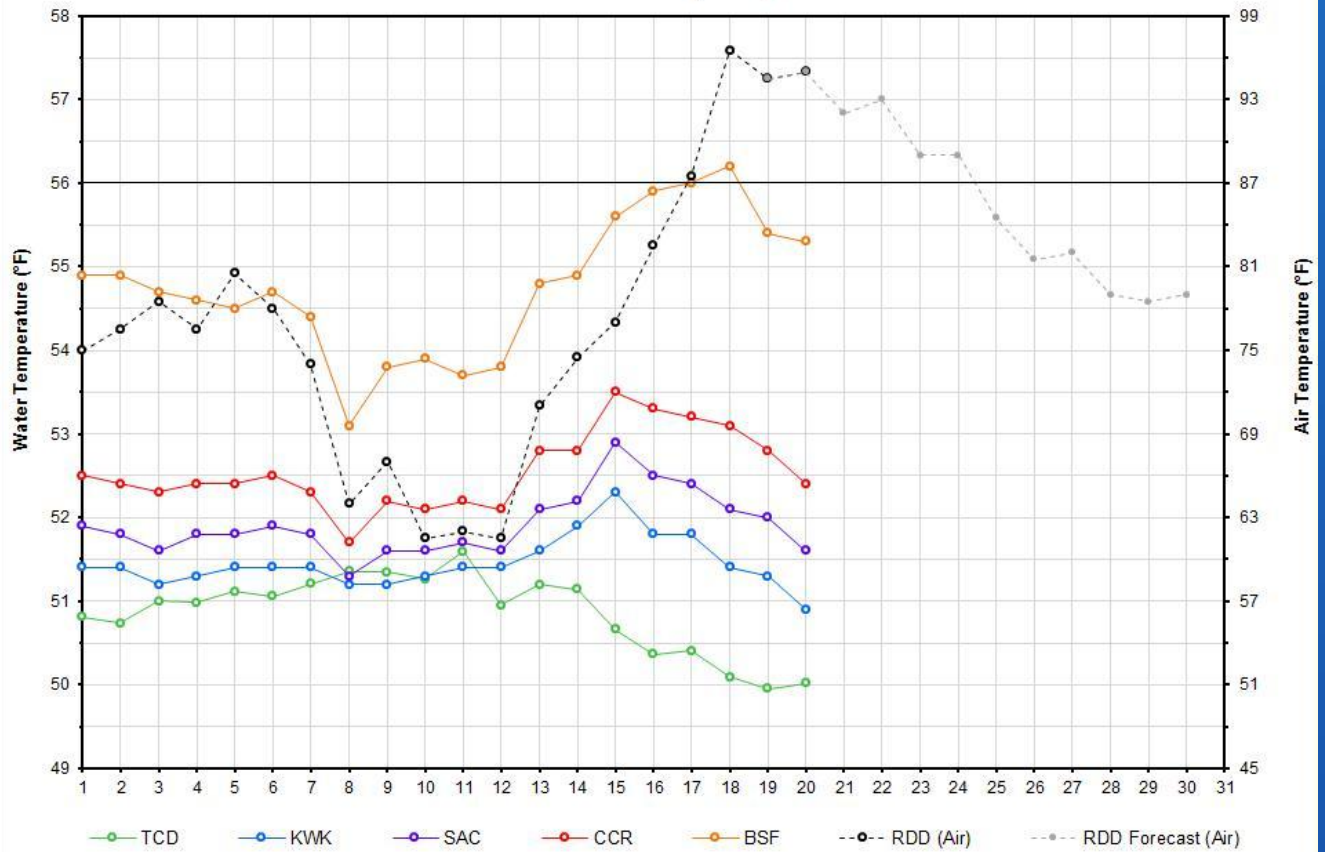
June Mean Daily Temperatures
